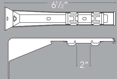
Double wall-mounted bracket
